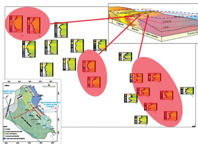
Fig. 3. The concept of the geological structure of the field (the areas of potential growth of organogenic structures are highlighted in color)
