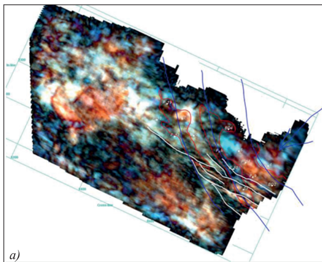
Fig. 5. Spectral decomposition
